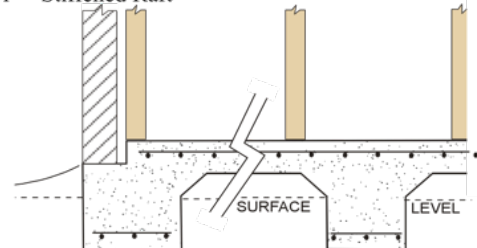
Fig. 1 Stiffened Raft
